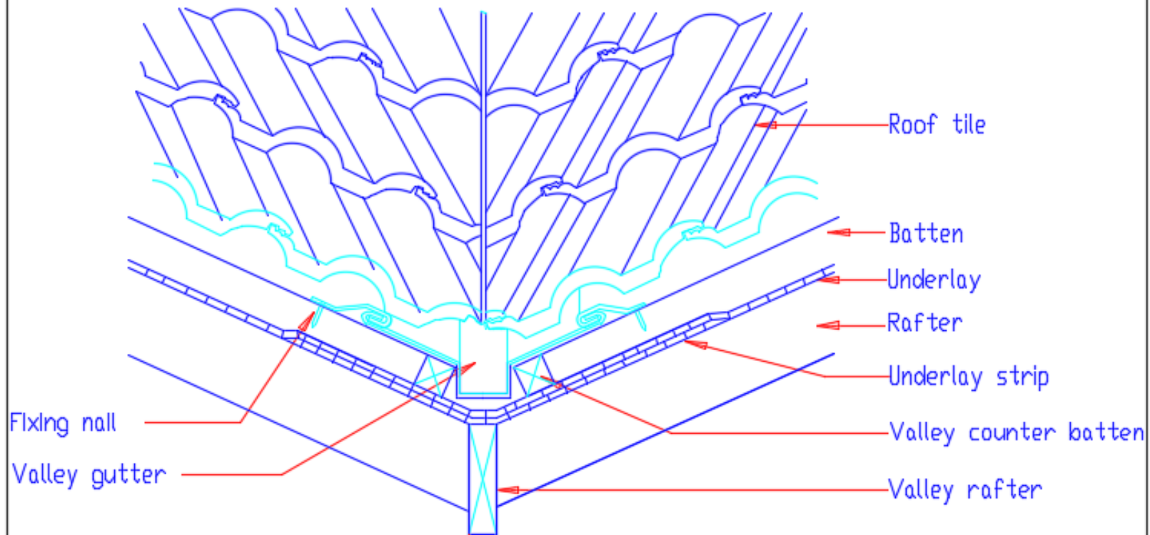
CLOSED VALLEY WITH PREFORMED GUTTER
