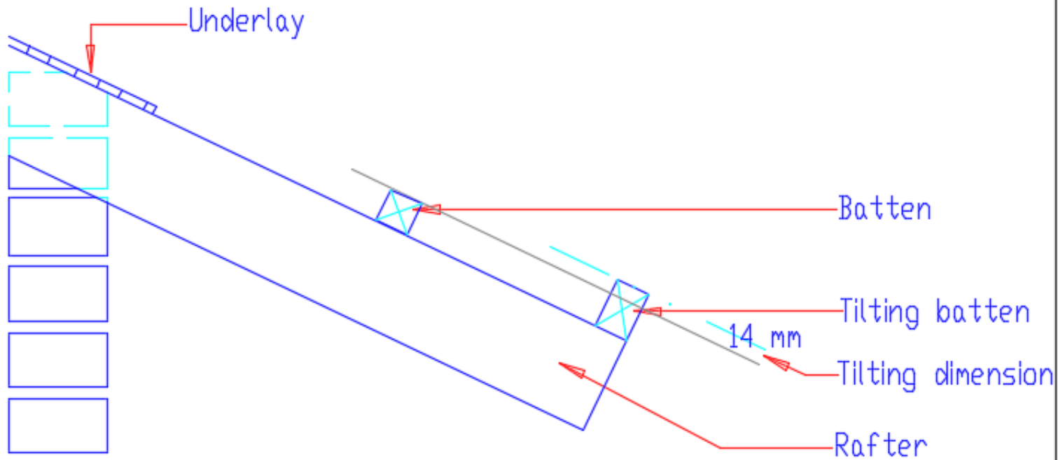
EAVES BATTEN POSITION WITHOUT FASCIA
