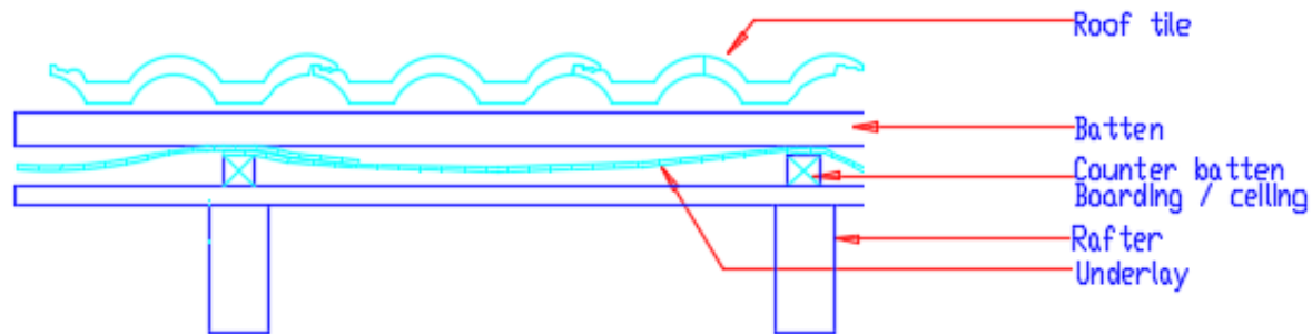
UNDERLAY OVER BOARDERD ROOF ILLUSTRATING LAPS
