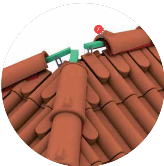
ADVANCE Premium Lusa 3 pitch roof
