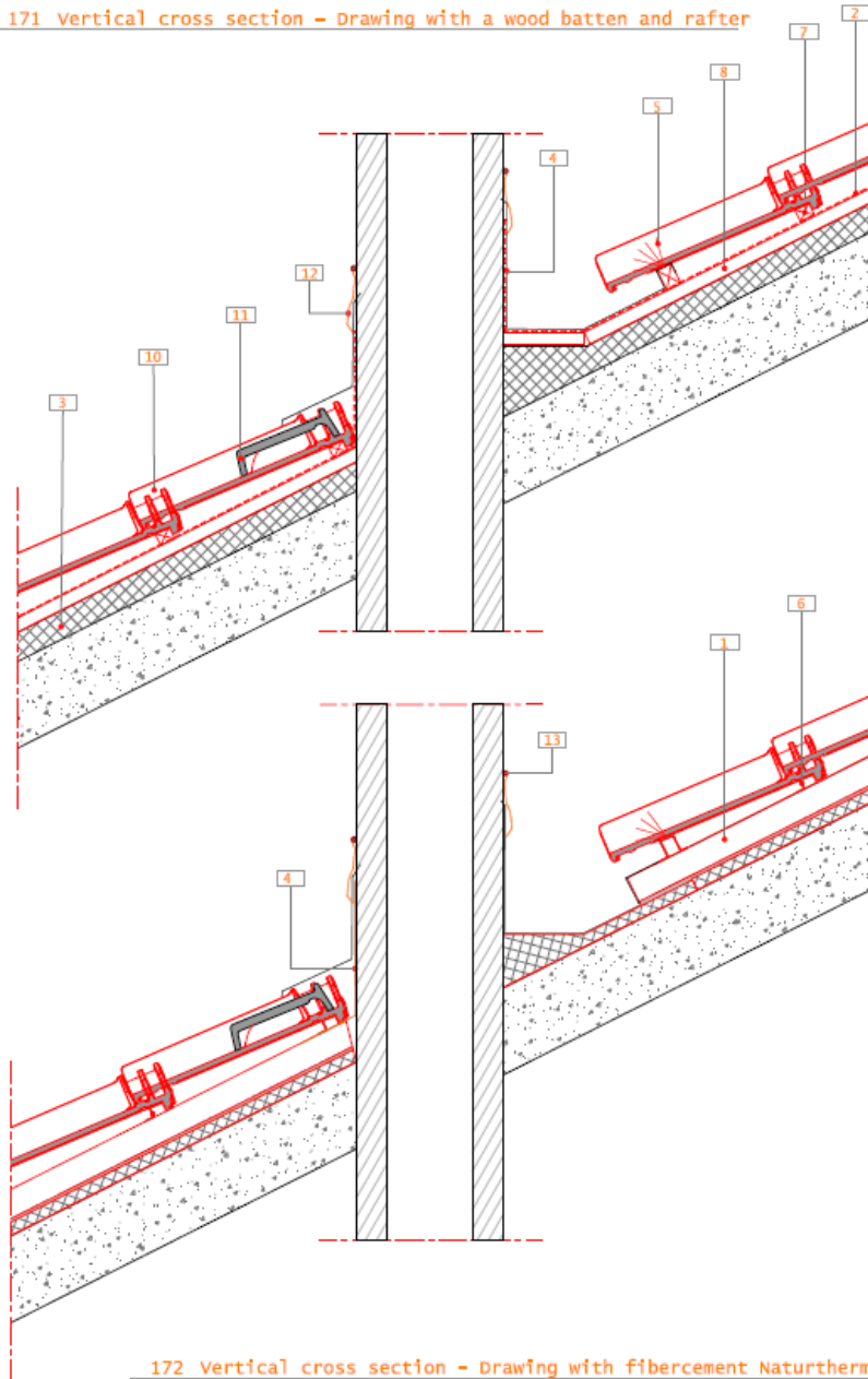
172 Vertical cross section - Drawing with fiber cement Naturtherm sheet
