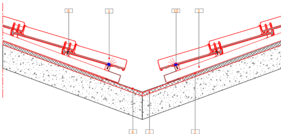
142 Vertical cross section - Drawing with fibercement Naturtherm sheet
