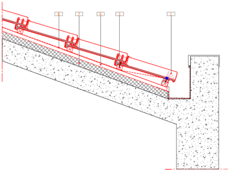
161 Vertical cross section - Drawing with a wood batten and rafter
