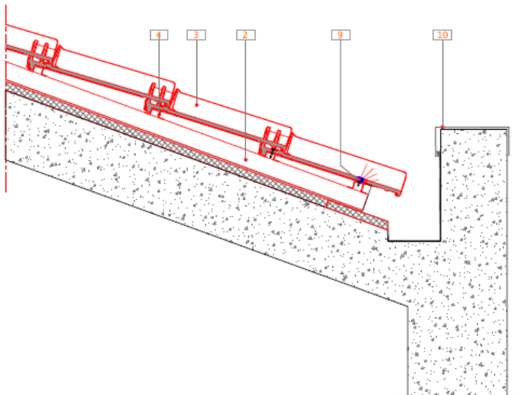
162 Vertical cross section - Drawing with fibercement Naturtherm sheet
