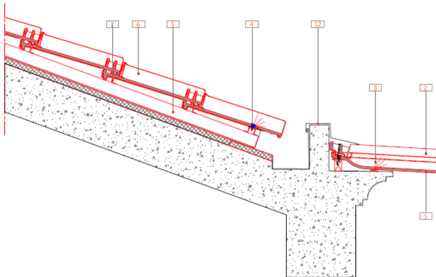
192 vertical cross section - Drawing with fibercement Naturtherm sheet
