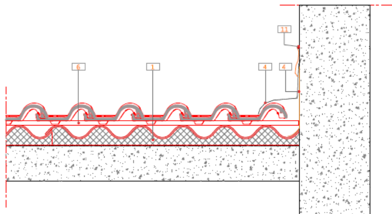
182 vertical longitudinal section - Drawing with fiber cement Naturtherm sheet
