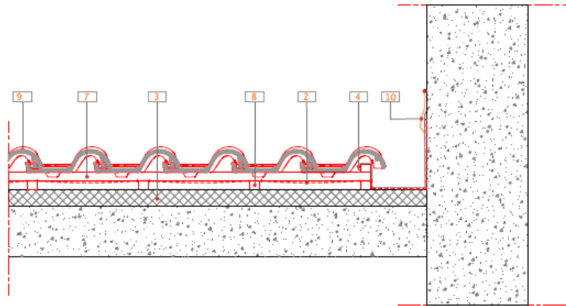
181 vertical longitudinal section - Drawing with a wood batten and rafter
