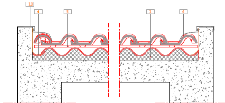
152 vertical longitudinal section - Drawing with fibercement Naturtherm sheet
