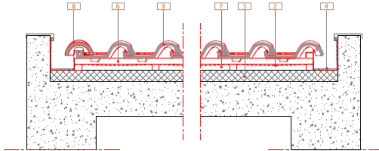
151 vertical longitudinal section - Drawing with a wood batten and rafter
